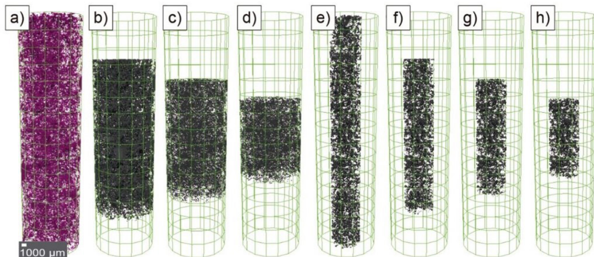
Figure 10. Candidate geometries for RVE of FAM (Souza et al., 2022)
