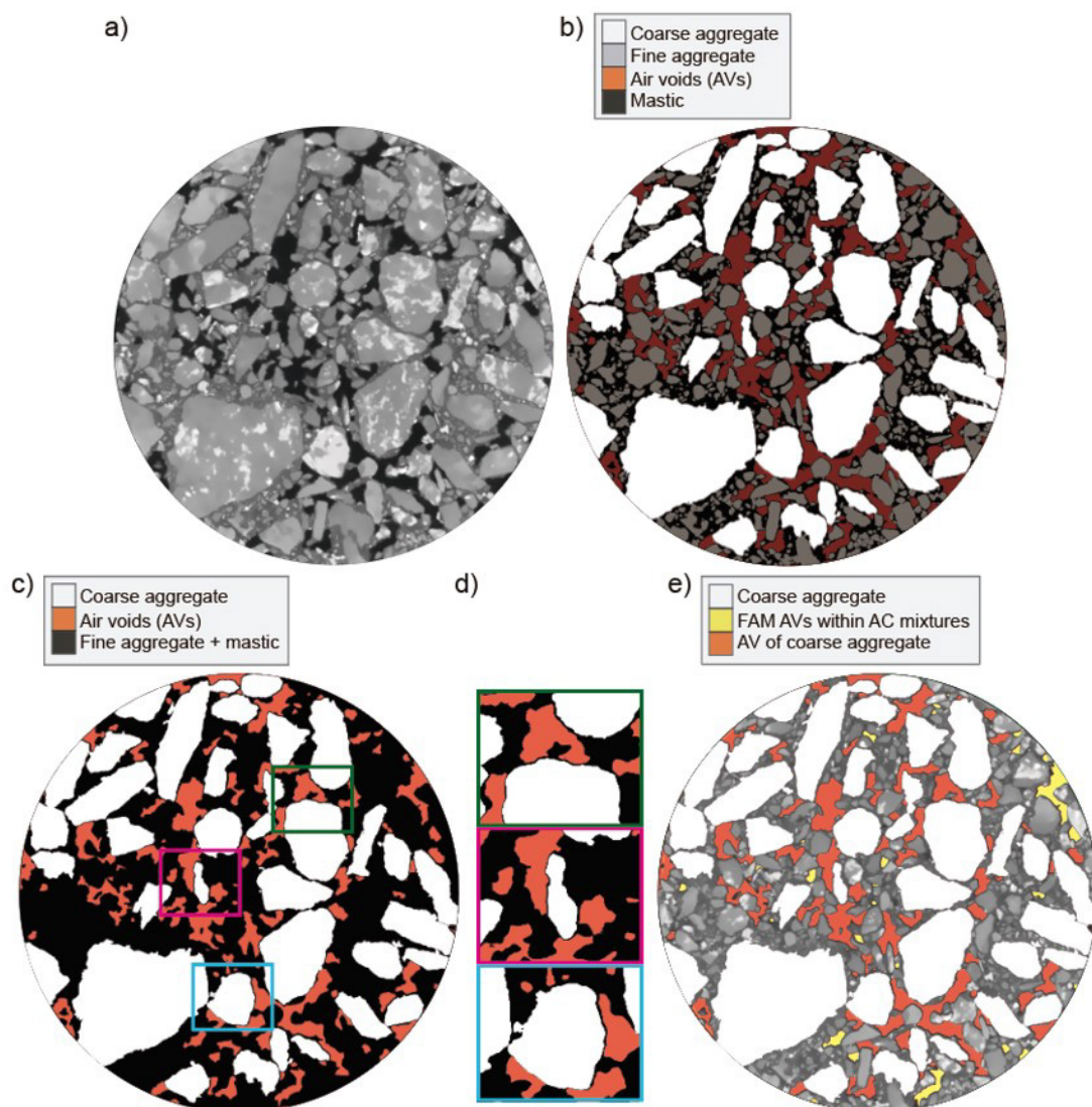
Figure 13. a) Cross section image of an AC, b) segmented image of coarse aggregates, fine aggregates, AVs, and mastic, c) AVs around coarse aggregates particles, d) details of AVs touching coarse aggregates, and e) different types of AVs in the microstructure of the AC
