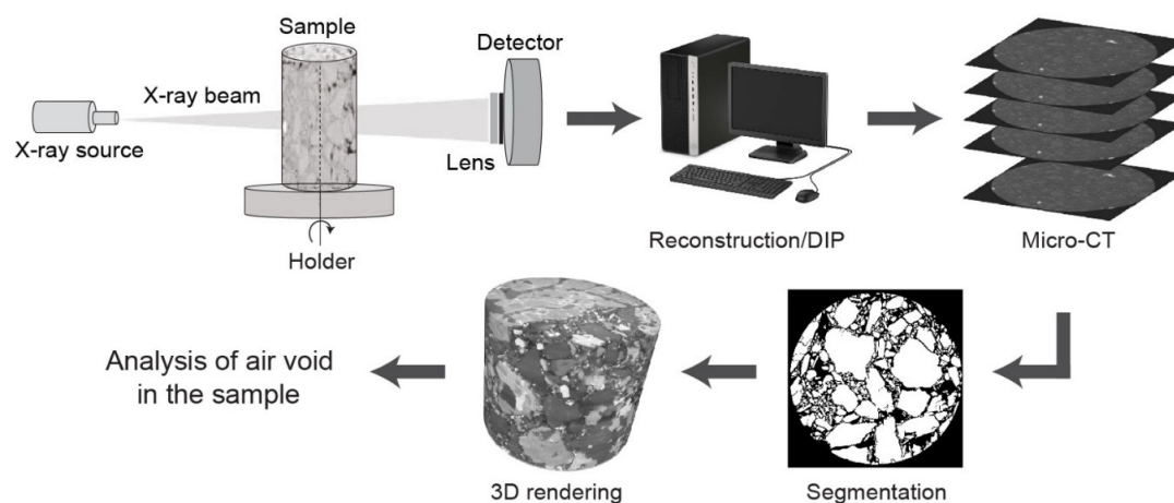
Figure 1. Illustration of the micro-CT process adopted to quantify the microstructural characteristics of asphaltic materials (adapted from Zelelew et al., 2013 and Tashman et al., 2002)
