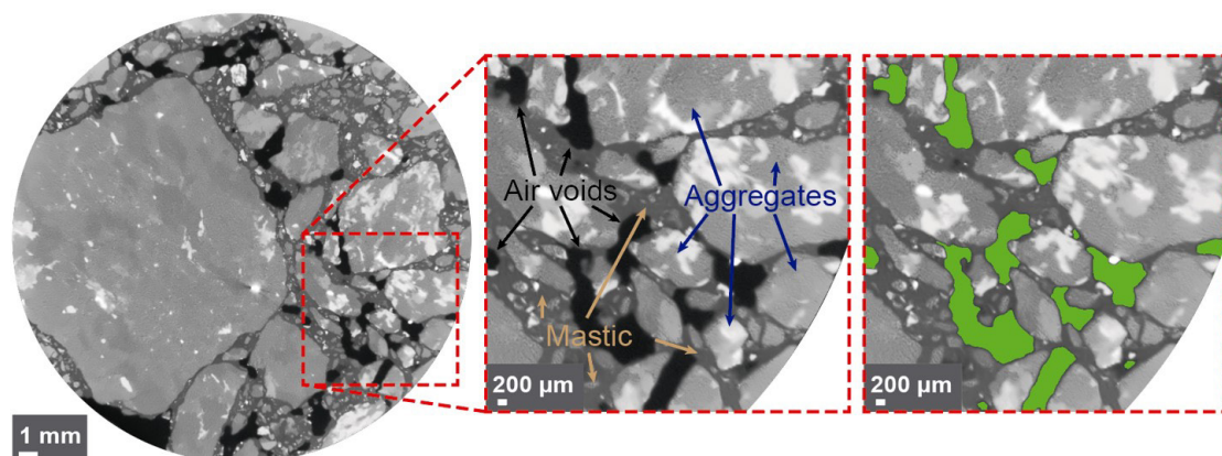
Figure 8. Segmentation of AVs in AC using the U-Net architecture (Enríquez-Léon et al., 2021)
