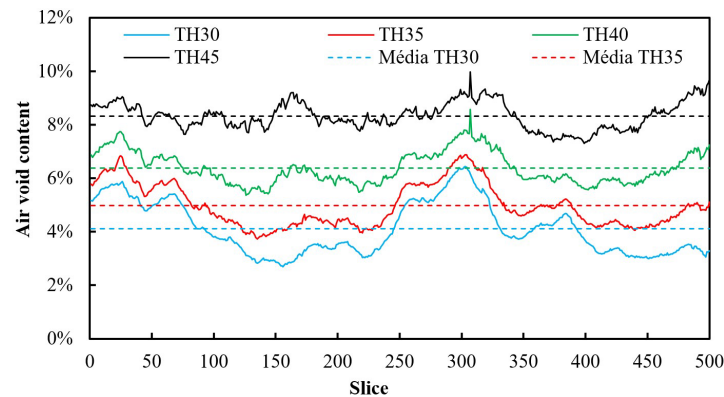
Figure 7. Distribution of AVs in an AC sample for different TH values
