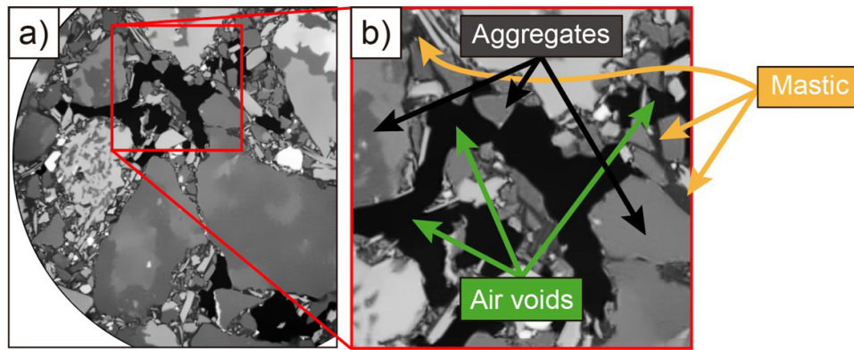
Figure 5. AC constituents: a) original image and b) amplified image
