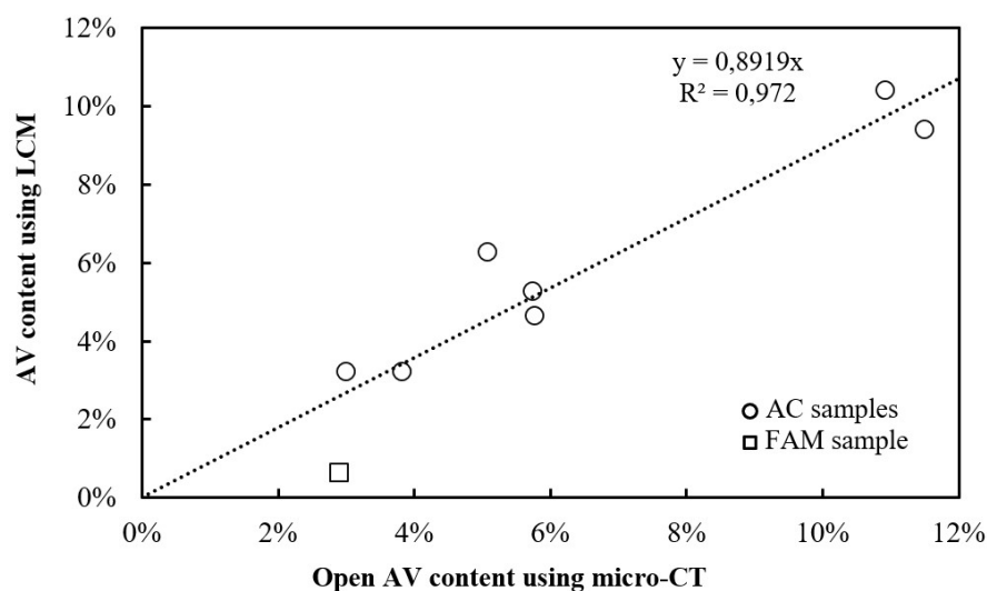
Figure 12. Correlation between open AV content obtained by micro-CT and LCM (Souza et al., 2022 and Enríquez-León et al., 2021)
