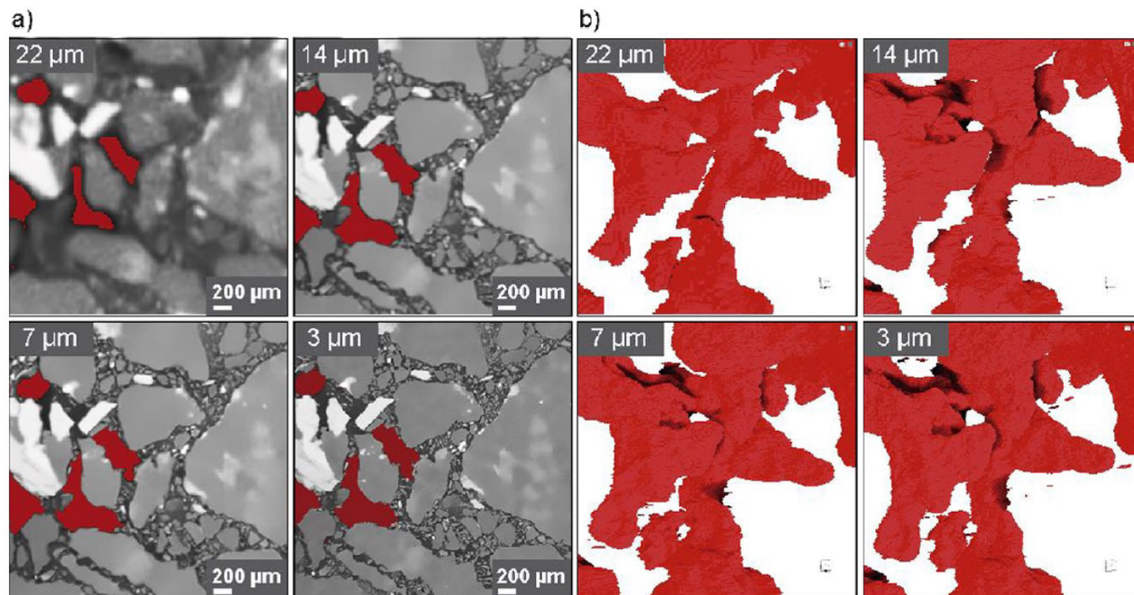
Figure 2. Effect of the spatial resolution on the characterization of AVs: a) cross sections and b) 3D rendered images
