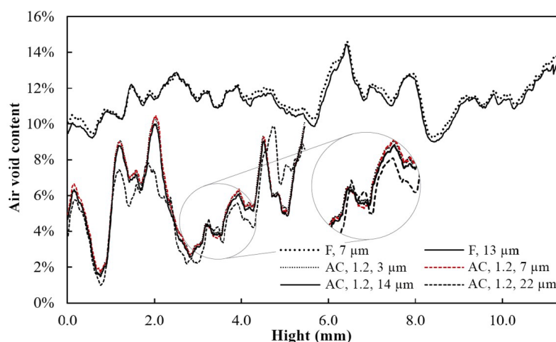
Figure 3. Characterization of AVs using different spatial resolutions in an AC sample (Enríquez-León et al., 2021)
