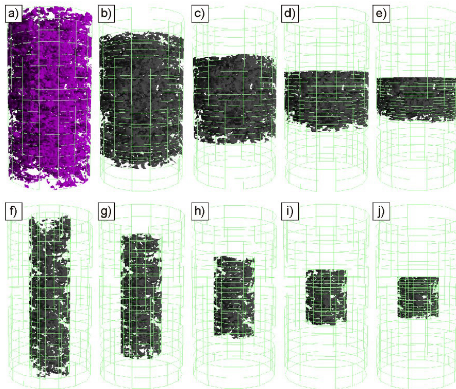
Figure 9. Candidate geometries for RVE of AC (Enríquez-Léon et al., 2021)
