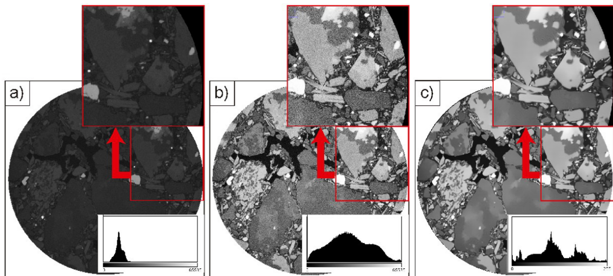
Figure 4. Example of pre-processing: a) original micro-CT image, b) pre-processed image with equalization, and c) pre-processed image with NLM filter
